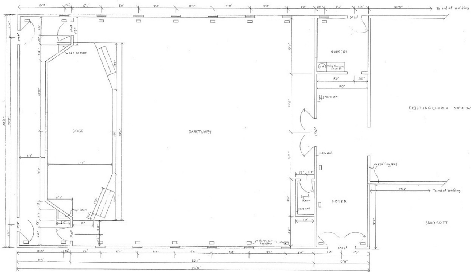
FLOOR PLAN 1/4" = 1'0"
